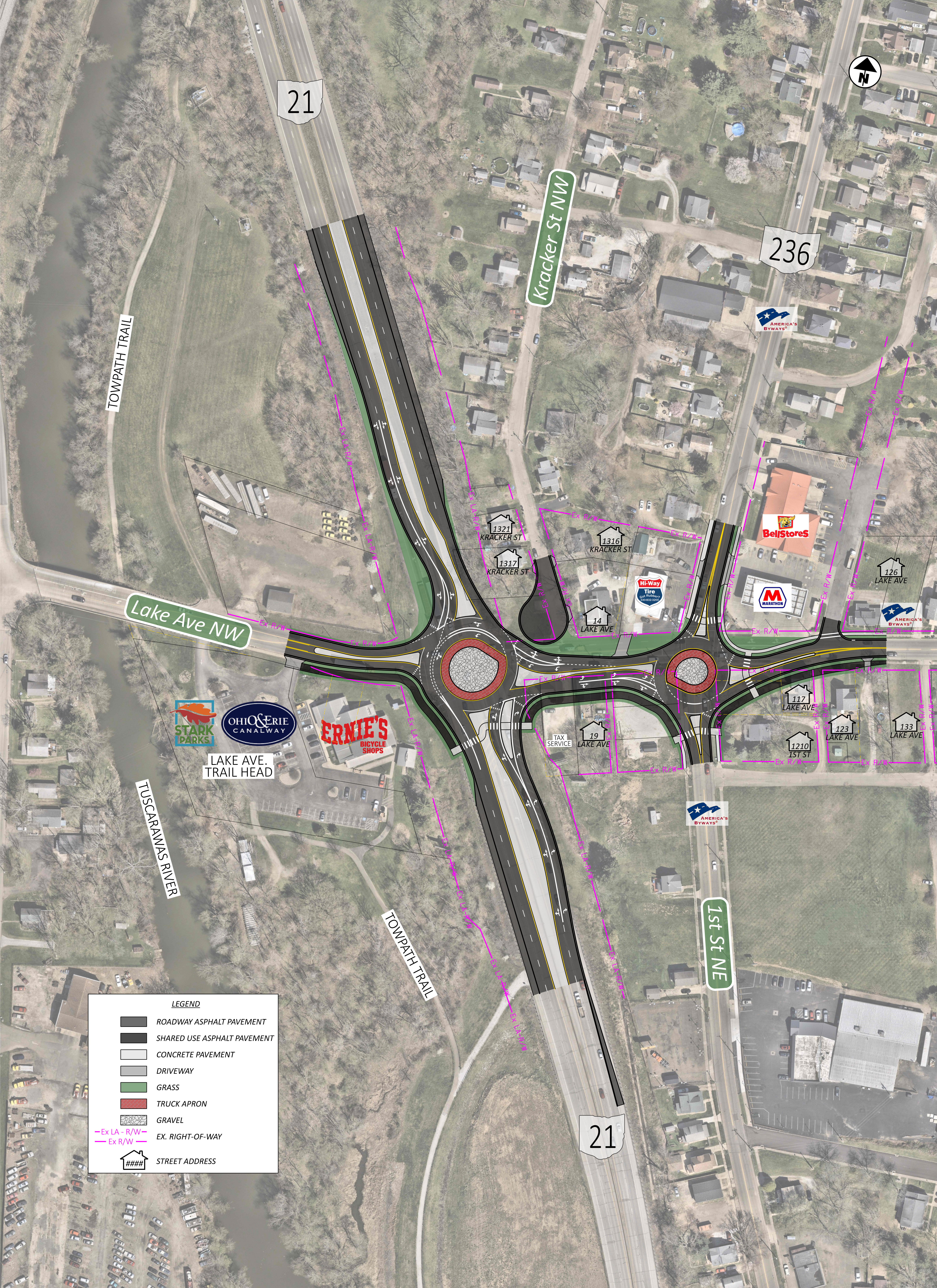
STA-21-10.46 SR-21 & LAKE AVENUE IMPROVEMENTS (PID 122272) ALTERNATIVE 2 (VIEW 1) ROUNDABOUT CORRIDOR WITH SHARED USE PATH
