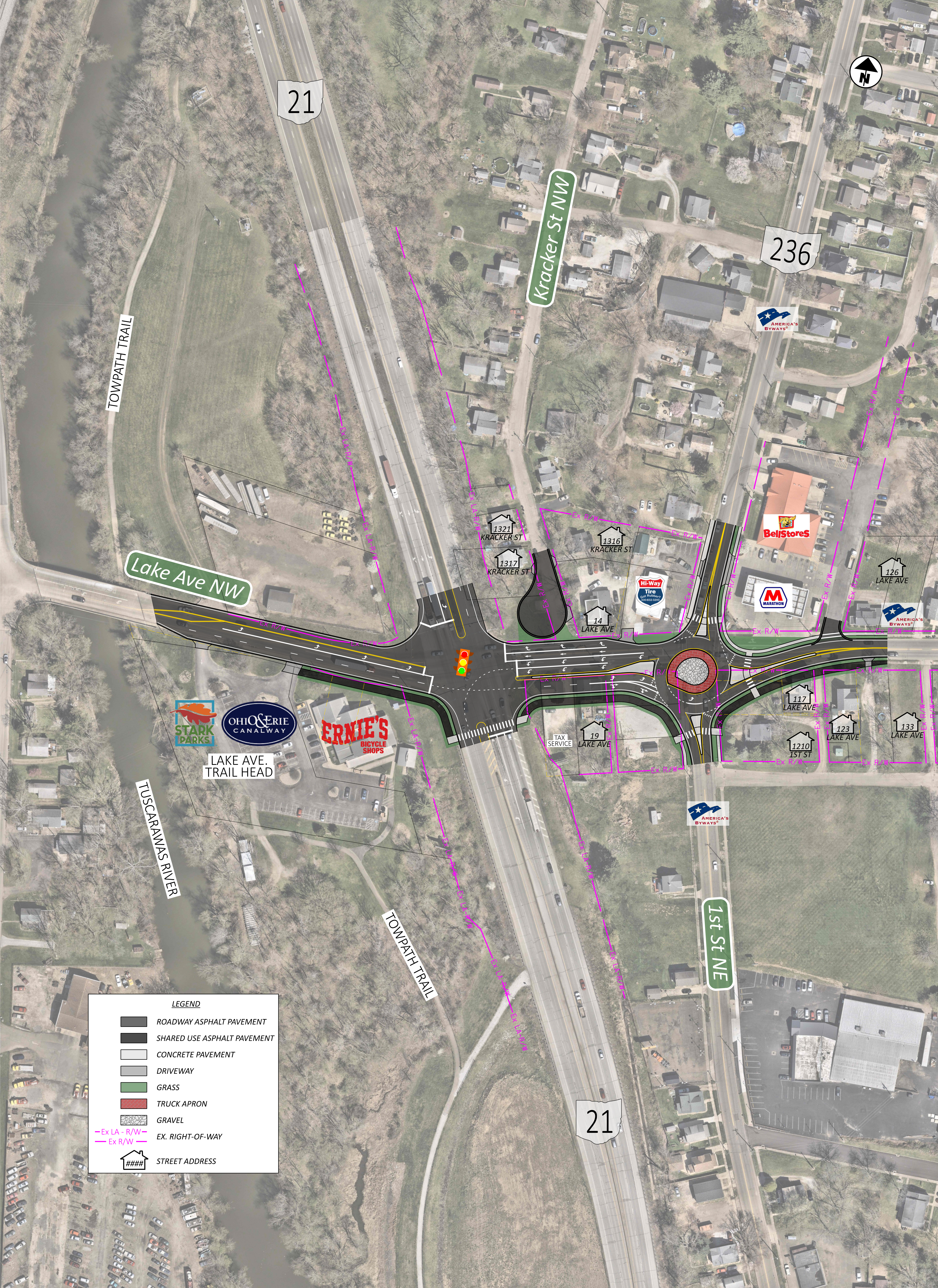
STA-21-10.46 SR-21 & LAKE AVENUE IMPROVEMENTS (PID 122272) ALTERNATIVE 5 (VIEW 1) TRAFFIC SIGNAL UPGRADES, ROUNDABOUT, AND ADDITIONAL TURN LANES WITH SHARED USE PATH
